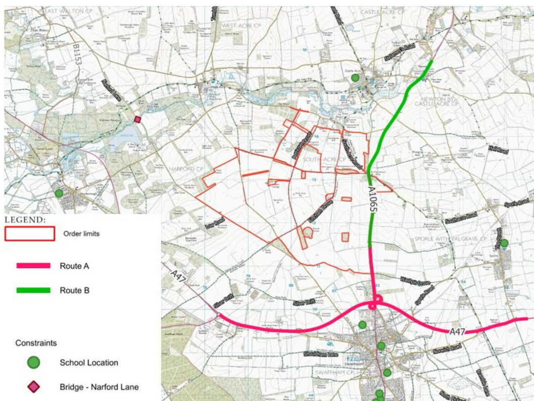
Figure 4-1 Proposed Routes for Construction Vehicles
